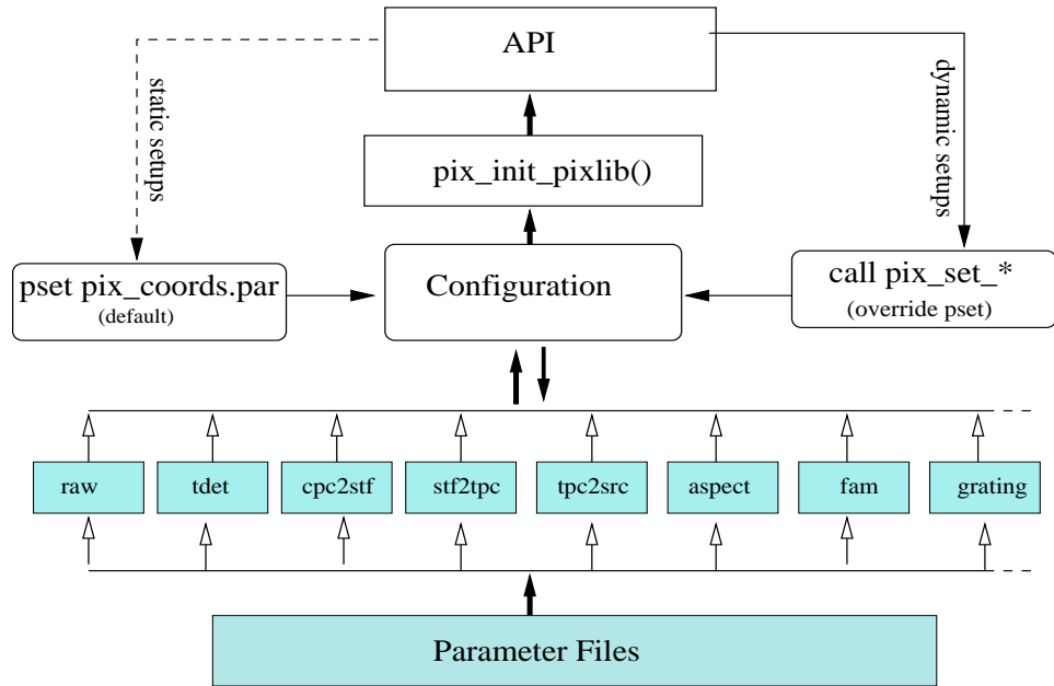
Figure 2. Pixlib data flow and system configuration. Each smaller box above represents a module. For example, the “raw” and “cpc2stf” boxes denote the modules of pix_raw.c and pix_cp2stf.c , respectively.
