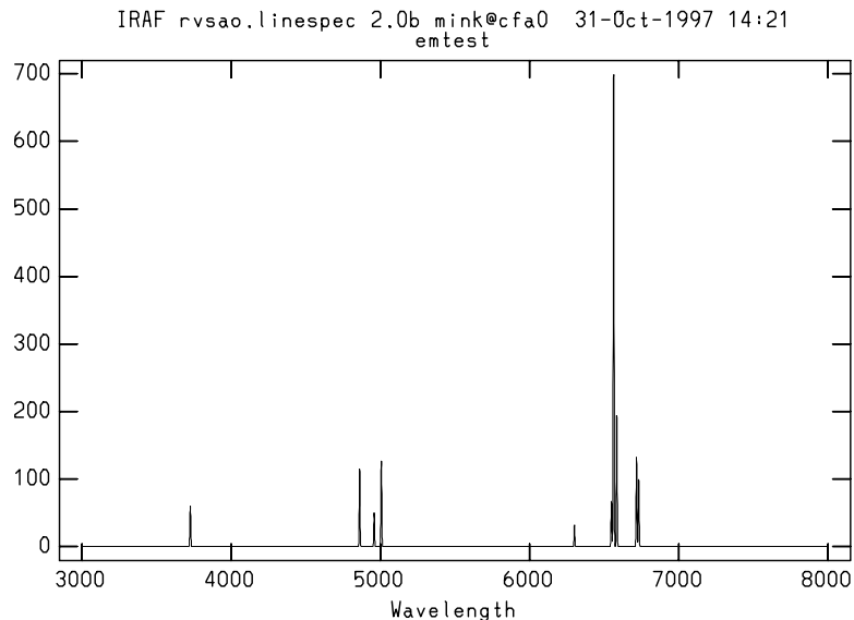
Figure 1. This is an artificial emission line spectrum created by LINESPEC for SAO's FAST Spectrograph
